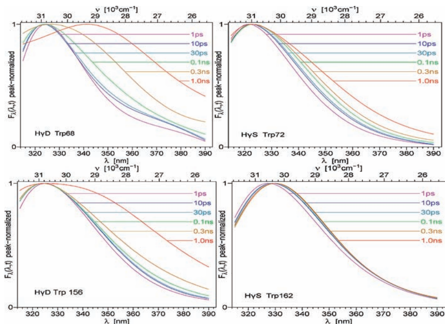
Figure 4. Time-resolved emission spectra (TRES) of \gamma -crystallins.
