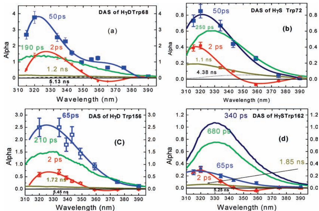
Figure 2. Decay associated spectra of Trp in crystallins.
