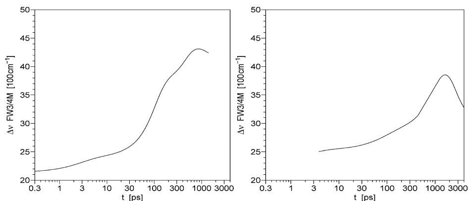
Figure 5. Energy width of (left) Trp68 \gamma D-Crystallin and (right) Trp72 \gamma S-Crystallin.
