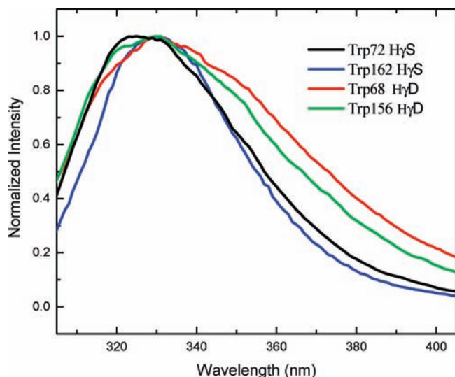
Figure 1. Steady state fluorescence of human \gamma -crystallins.
