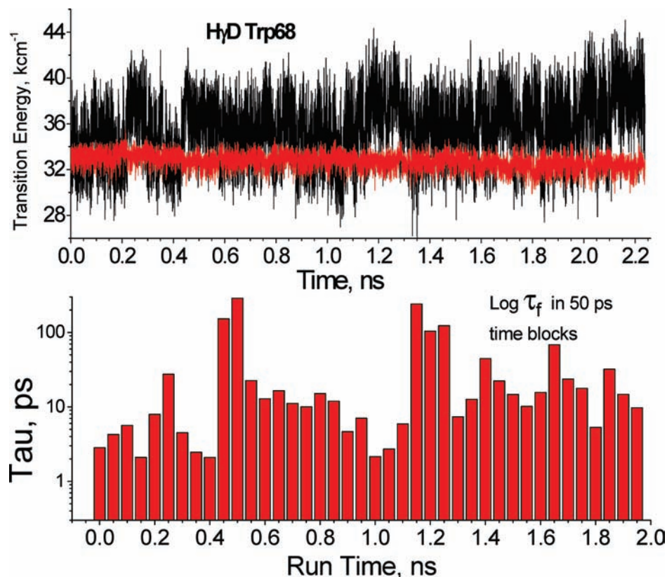
Figure 6. Top 2.2 ns QM-MM simulation of lowest CT (black) and ^1L_a (red) state transition energies for Trp68 \gamma D-Crystallin with points shown every 1 ps. Bottom: Sequential 50-ps \log_{10} average lifetimes based on the corresponding CT- ^1L_a energy gaps in the top figure. The heterogeneity suggested by the plot is consistent with that seen in the observed lifetimes.
